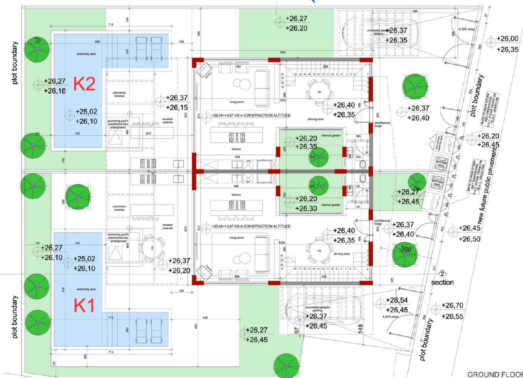
GROUND FLOOR
