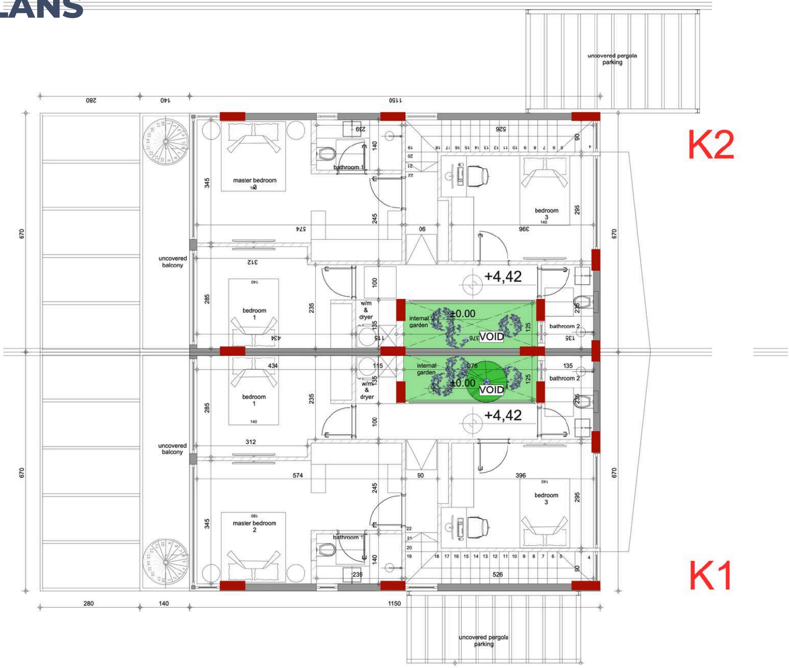
FIRST FLOOR
